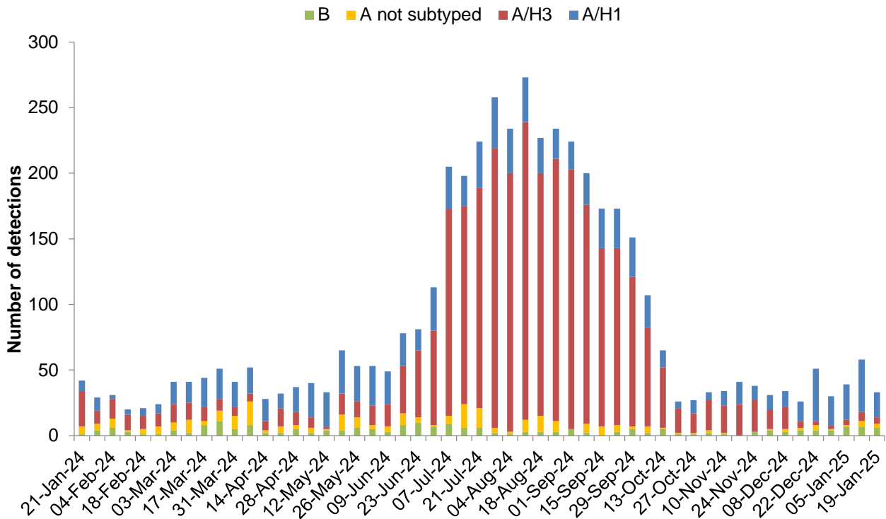
Figure 6. Number of PCR positive influenza detections at PathWest by type, subtype and week, WA, 2024 to 2025 YTD
