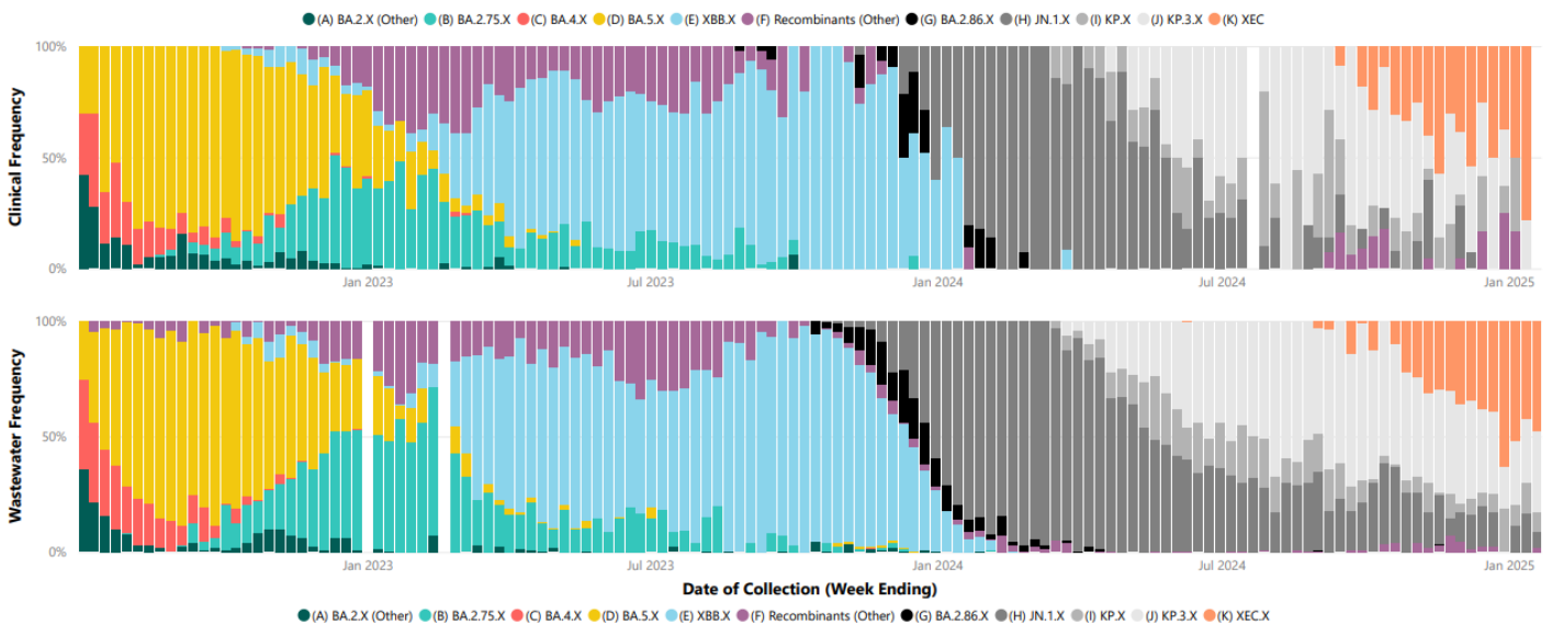
Figure 12. Distribution of SARS-CoV-2 variants in clinical samples (top) and metropolitan wastewater catchments (bottom), 03 July 2022 to 10 January 2025.
